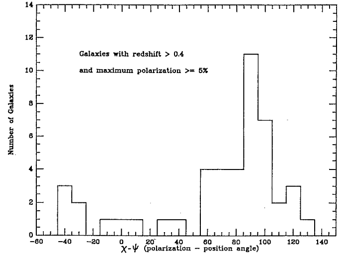
FIG. 2. A histogram of number of galaxies vs \chi - \psi , in bins of 10^\circ , for those sources with p_{\max} \geq 5\% and z > 0.4 . The peak near 90^\circ is obvious.
